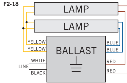
FOR 1 LAMP OPERATIONS, CAP 1 YELLOW LEAD
