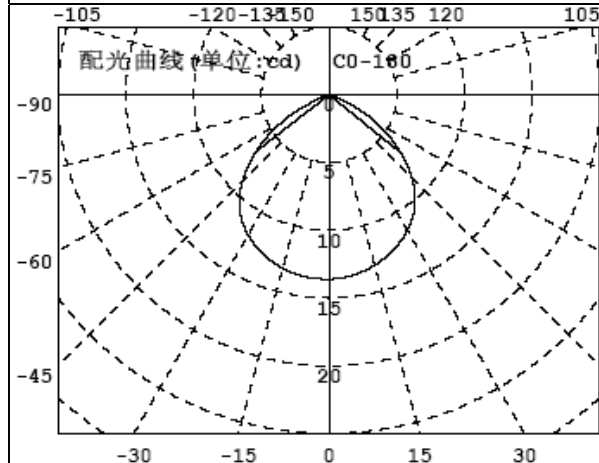
Polar Candela Plot
