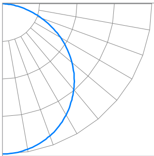
BLP24/PS50/FCCT (Typical performance @ 50W, 4000K)
