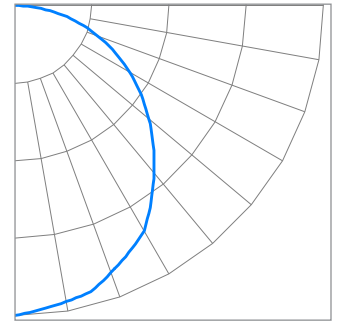
BLP22-37/30W/8xx (Typical performance @ 3500K)
