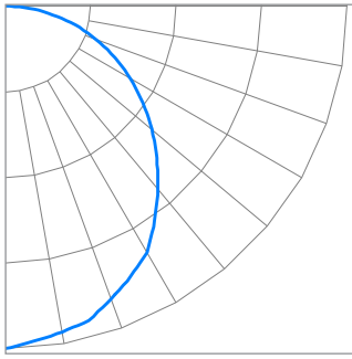
BLP24-44/40W/8xx (Typical performance @ 4000K)
