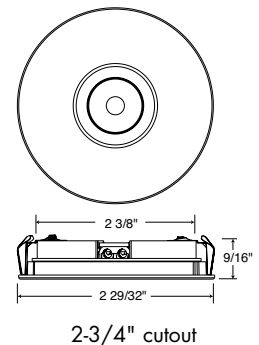
Recessed Mount (USTLR1)
