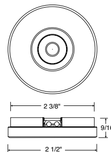
Surface Mount (USTL1)
